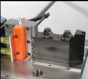
Shearing Tool
